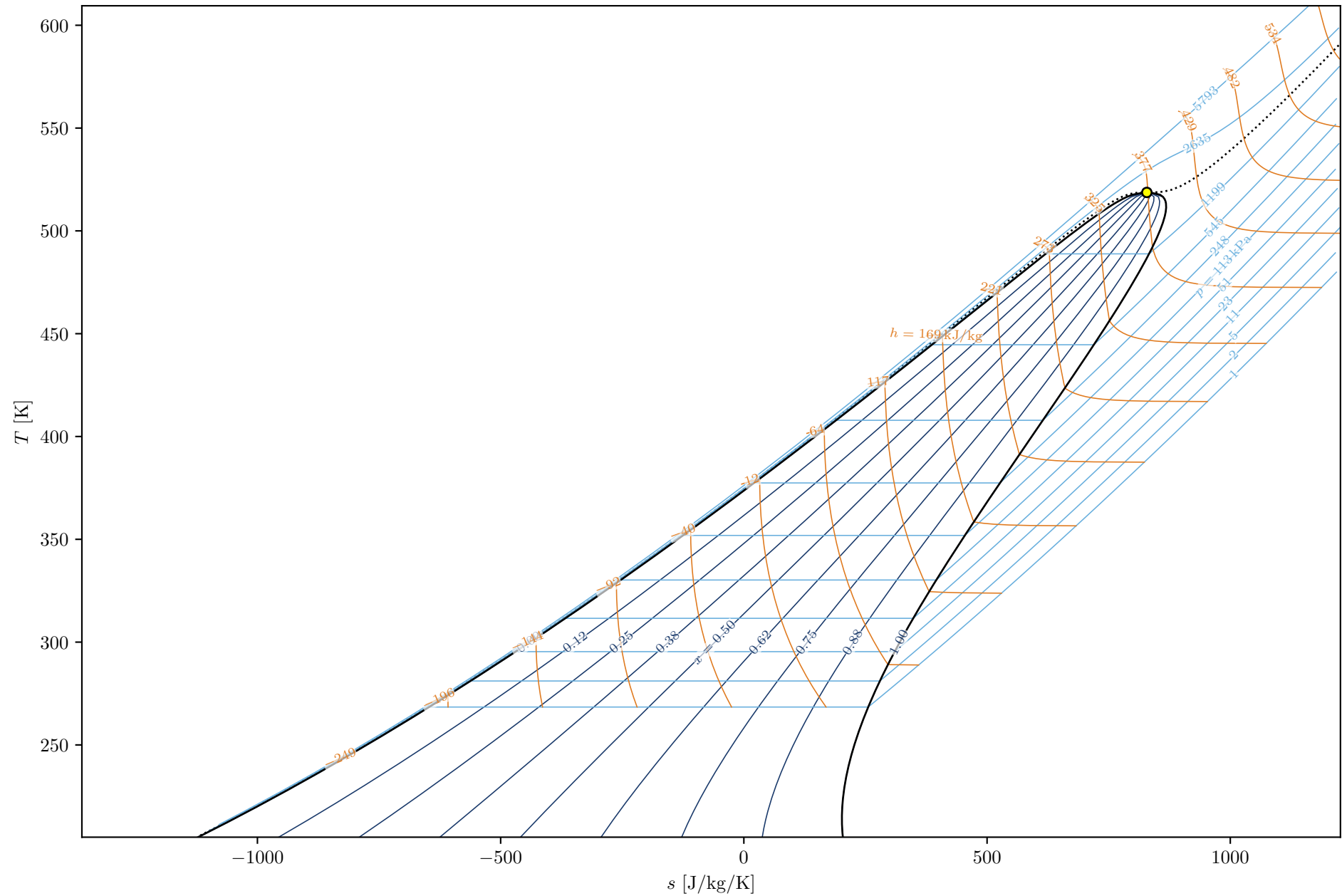
Thermodynamic Diagram (TS) – MM
